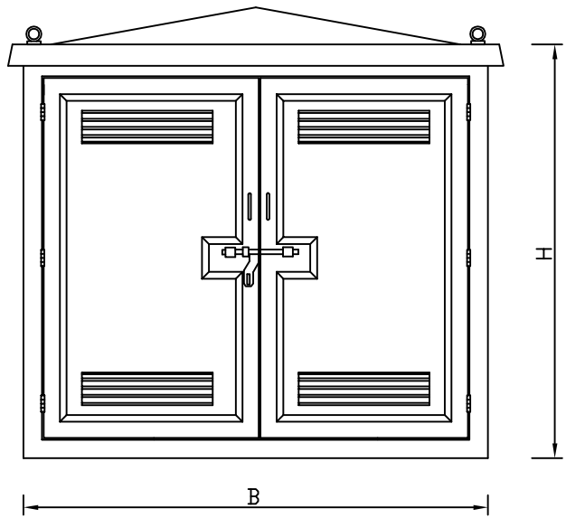
FRONT/ REAR ELEVATION
