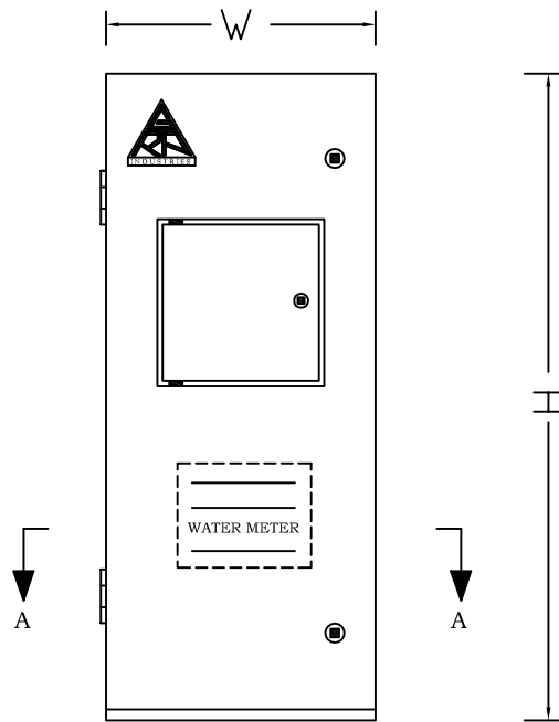
FRONT ELEVATION
